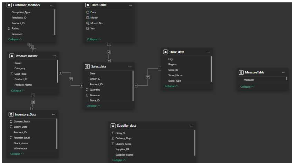
Figure: Data Model and Table Relationships
